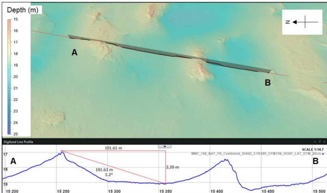
Plate 1.31 A profile along the route between KP 10 and KP 10.5 over a sample of the outcrops in the area. The outcrops stand >2 m above the surrounding seabed (MMT, 2022)
